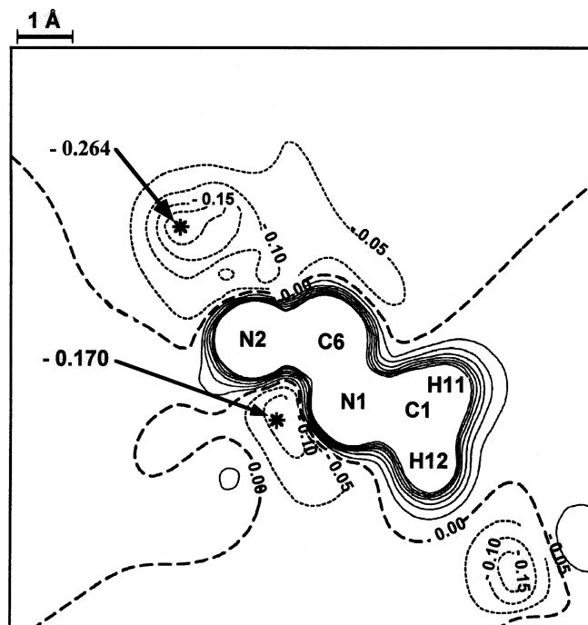
Figure 2. Experimental molecular electrostatic potential [eÅ -1 ] of 1,4,8,11-tetraazatricyclo[9.3.1.1 4,8 ]hexadecane in the (C6–N1–C1) plane
