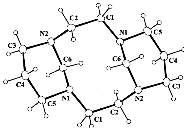
Figure 1. ORTEP view and numbering scheme of 2 with 50% probability thermal ellipsoids for non-H atoms
